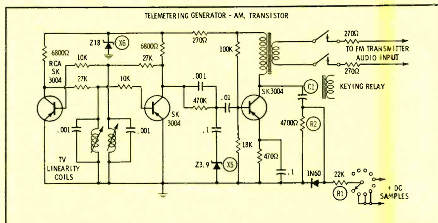
Fig. 18. Transistorized generator unit is used primarily for AM type of telemetry.
