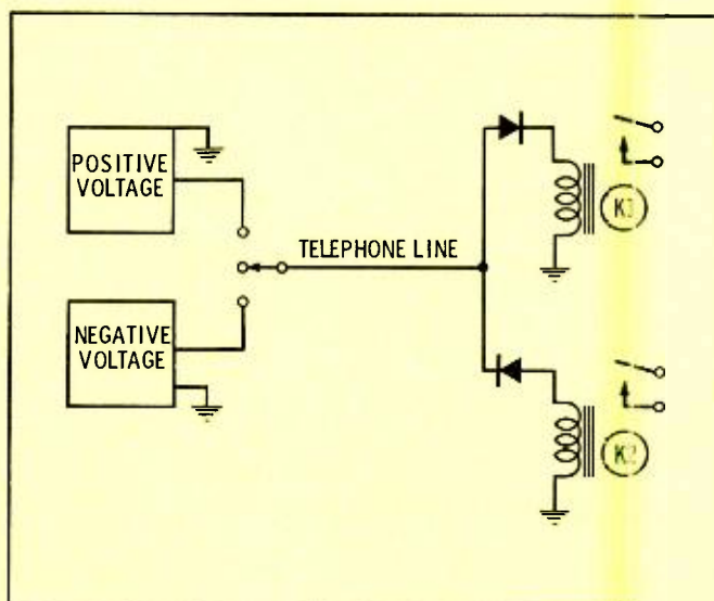
Fig. 3. Polarity-differential metering used in a remote system.
