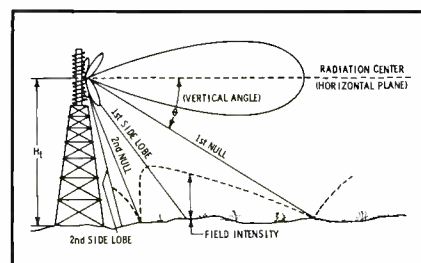
Fig. 6. Vertical nulls affect coverage.
