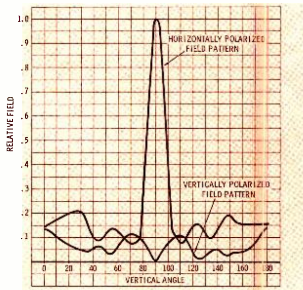
Fig. 3. Typical vertical pattern of single-bay helical antenna.
