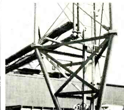
WTWO's 1000' main transmitting tower is just outside transmitter-room door.
