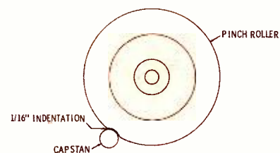
Fig. 2. Pressure exerted by pinch roller can be estimated from indentation.
