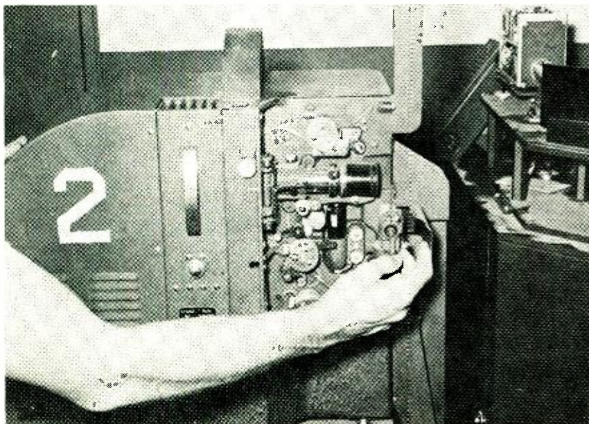
Fig. 5. View of film projector showing location of sound photocell and exciter.
