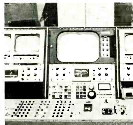
Video switching position. Lower knob below A-scope selects audio switch mode.
