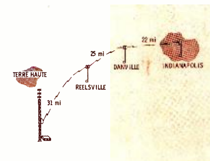
Fig. 3. A three-hop microwave system brings network programs to the station.
